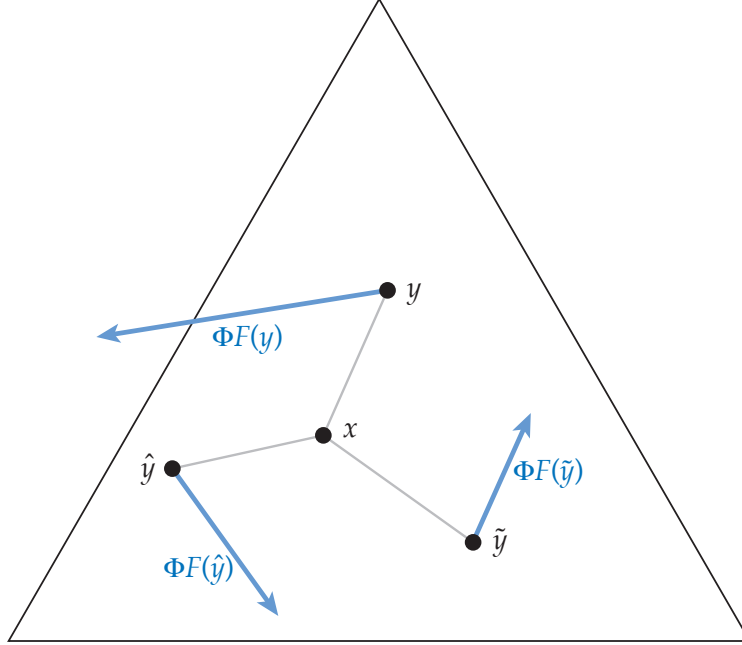
Figure 1: The geometric definition of GESS.
