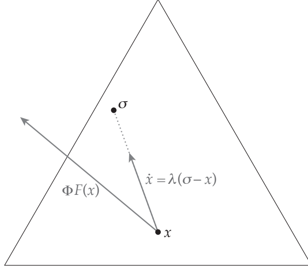
Figure 2: Target dynamics and positive correlation.
