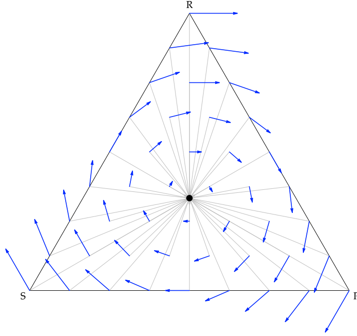
Figure 3: Payoff vectors and GNSS in standard RPS.
