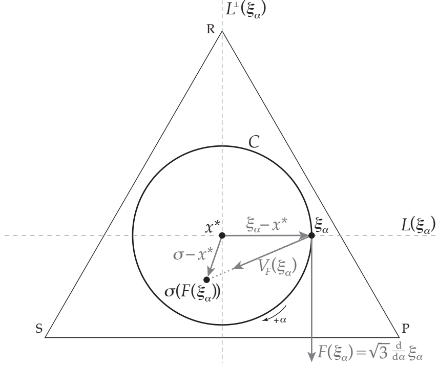
Figure 4: Integrability and inward motion of EPT dynamics in standard RPS.
