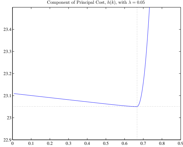
FIGURE 1. The function h(k) from the principal’s cost function with \lambda = 0.05 . The dotted lines show the optimal choice k_0^* = \rho\theta/(\rho + \lambda) and its corresponding value h(k_0^*) .
