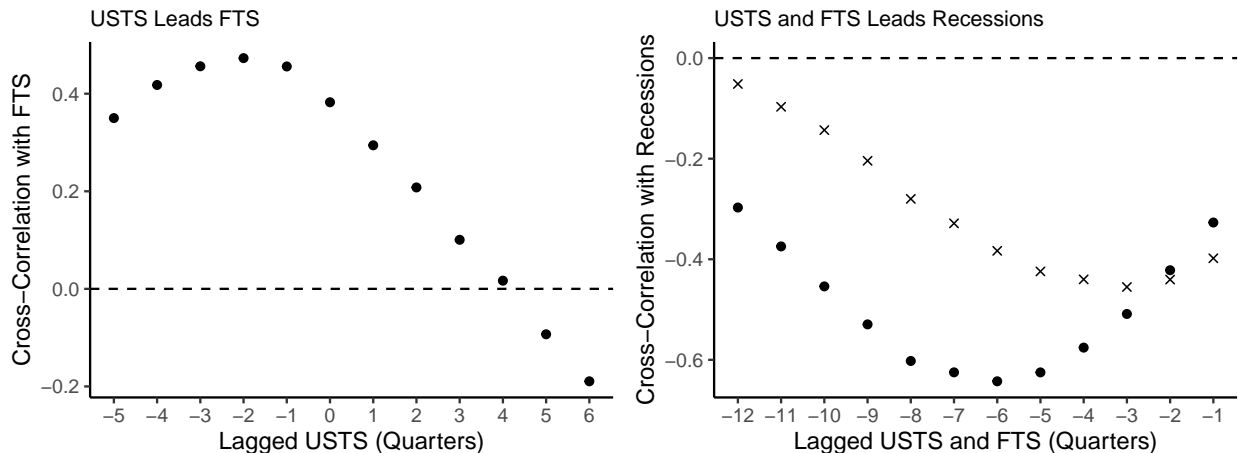
Figure 3: Cross-Correlation Coefficients
