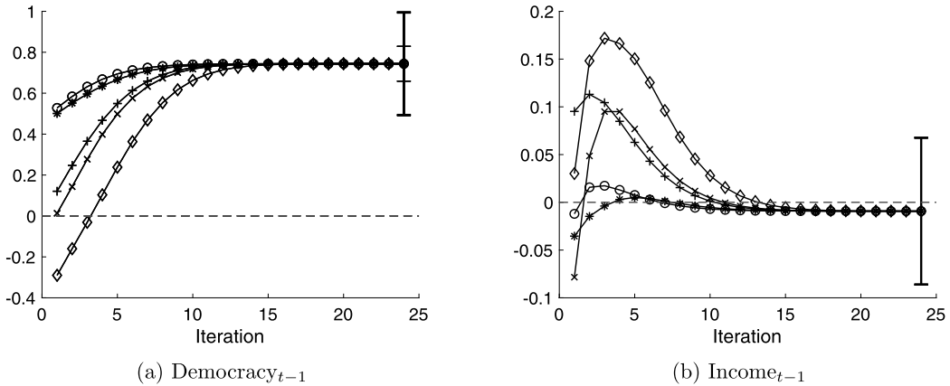
FIGURE 1.—Convergence path of the iterated GMM estimator in Column II of Table III with initial weight matrices \bar{W}_k(\tilde{\phi}) where \tilde{\phi} is the one-step GMM of AJRY (circle); \tilde{\phi} is the one-step GMM using the identity matrix (x); \tilde{\phi} = (0, 0, \dots) (+); \tilde{\phi} = (0.5, 0.5, \dots) (*); \tilde{\phi} = (-0.5, -0.5, \dots) (diamond), Thicker (lighter) error bar at the converging point is the asymptotic 95% confidence interval based on the robust (conventional) standard error.
