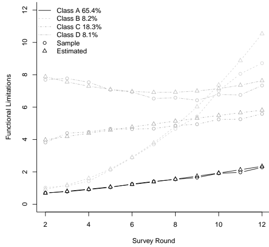
Figure 3: LCGA: Four Class Model with Quadratic Slope (n=9706)
