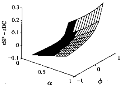
FIG. 4.—Difference in R & D shares: social optimum vs. the decentralized economy. Source: Author's calculations. The labor share ( \alpha ) ranges from .2 to .85 in the figure. Negative values are shaded.
