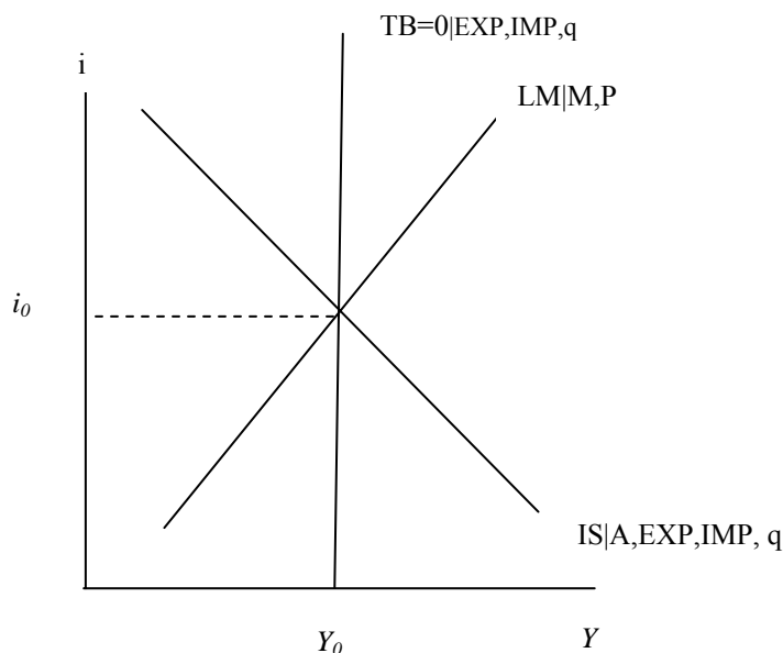
Figure 1: IS-LM-TB=0 in equilibrium
