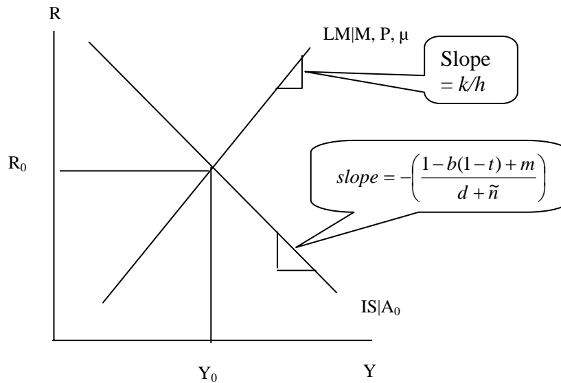
Figure 2: Equilibrium in IS-LM
