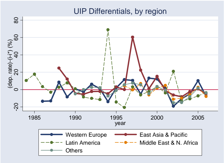
Figure 4: UIP Differentials for Different Regions (unbalanced)
