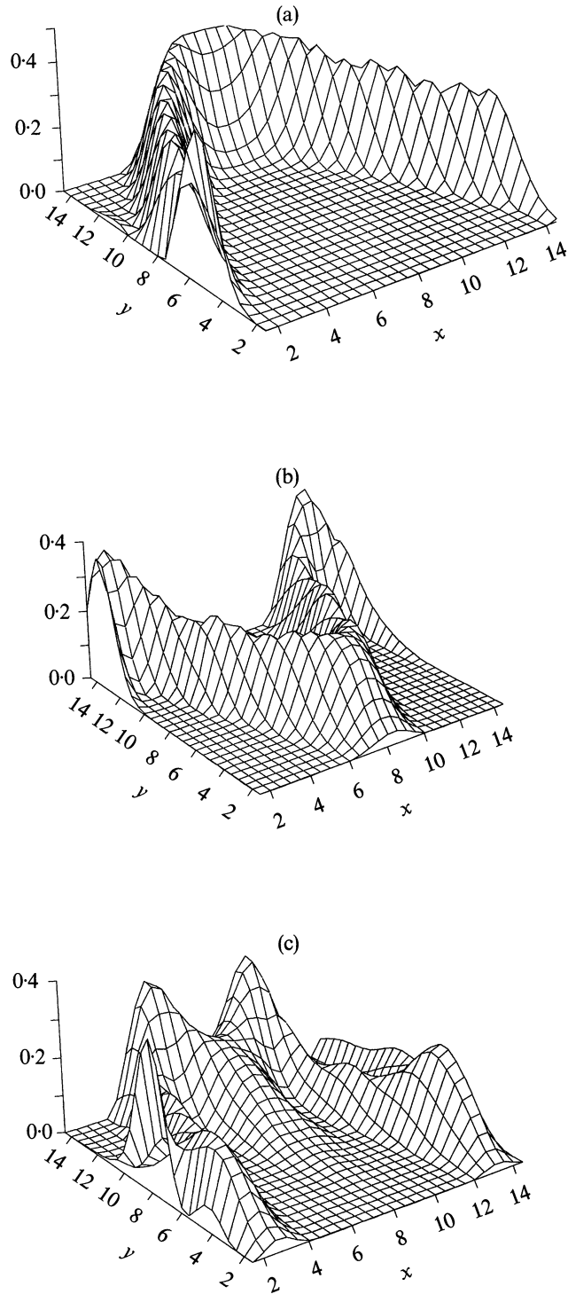
Fig. 1. The estimated g_m(y|x) for Example 1: the conditional density function of Y_{t+m} given Y_t = x for the logistic model (2.9). (a) m=1 , (b) m=2 , (c) m=3 .
