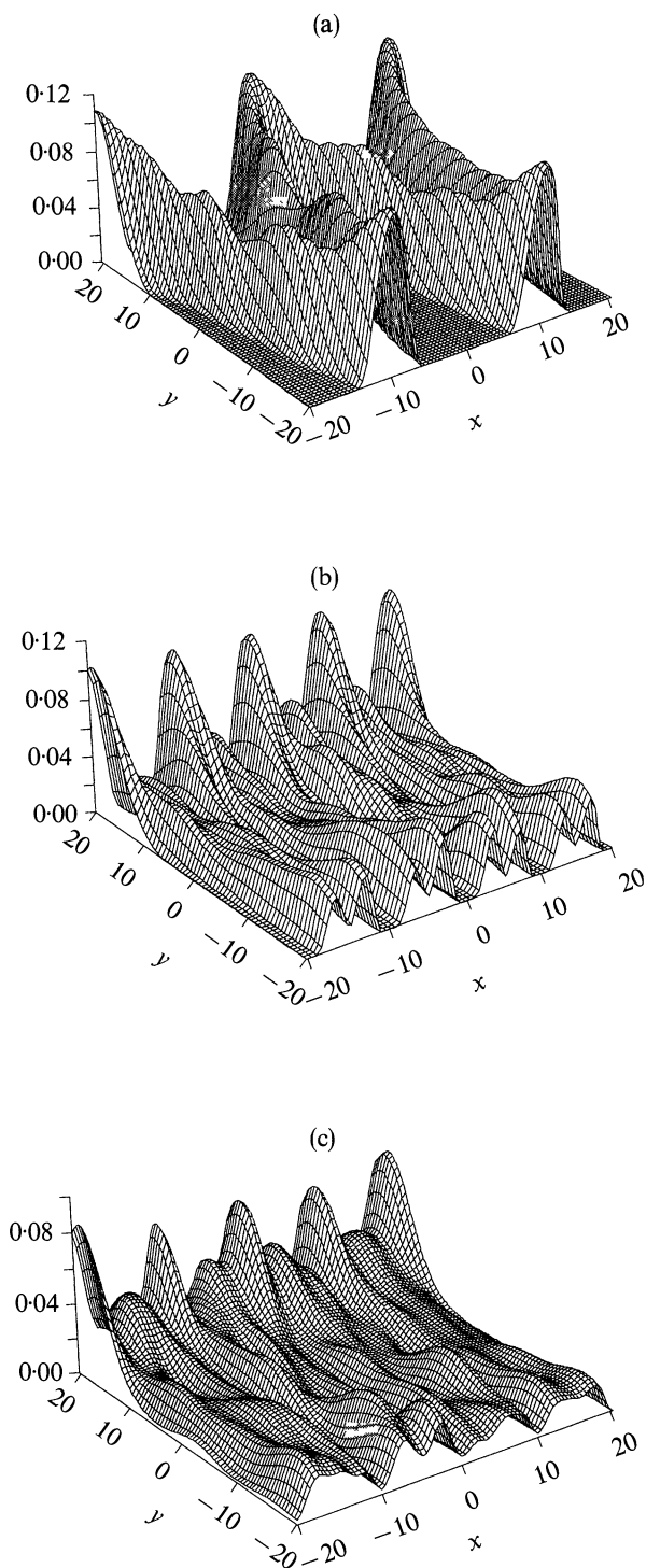
Fig. 2. The estimated g_m(y|x) for Example 2: the conditional density function of Y_{t+m} given Y_t = x for the cosine model (2.10). (a) m = 1 , (b) m = 2 , (c) m = 3 .
