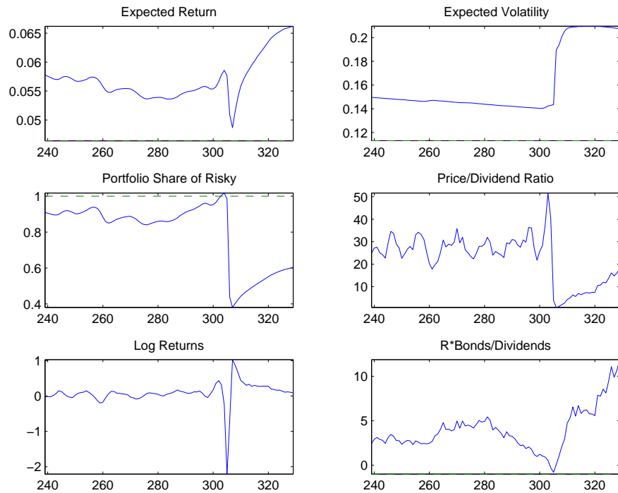
FIGURE 6. Detail of a simulation with constant gain \varepsilon = 0.003 . The top left panel plots m_t , the top right plots s_t , the middle left plots v_t , the middle right plots P_t/D_t , the bottom left panel shows \log R_t , and the bottom right panel plots RB_{t-1}/D_t .
